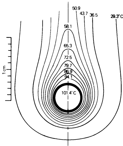
c. Measured isotherms around a cylinder in air when Gr_D \approx 585 (from [8.9]).
