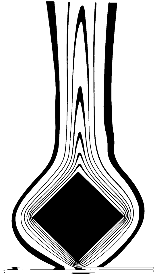
b. A square cylinder with a fairly low value of Gr . (Rendering of an interferogram shown in [8.9].)
