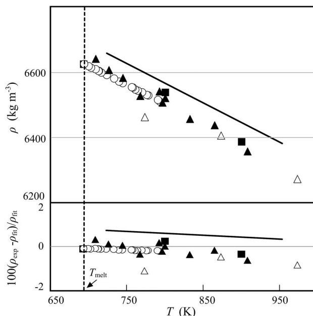
FIG. 7. Primary density data and their percentage deviations from Eq. (1) for liquid zinc as a function of temperature. Stankus and Khairulin 50 (■), Karamurzov 7 (—), Thresh 55 (○), Lucas 46 (▲), Gebhardt et al. 56 (Δ).
