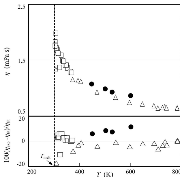
FIG. 10. Primary viscosity data and their percentage deviations from Eq. (2) for liquid gallium as a function of temperature. Tippelskirch 91 (Δ), Genrikh et al. 92 (□), Menz and Sauerwald 83 (●).
