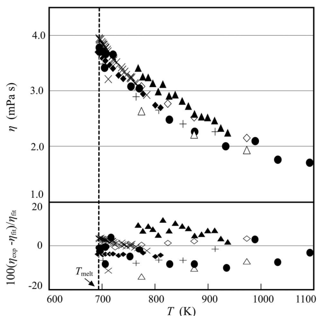
FIG. 15. Primary viscosity data and their percentage deviations from Eq. (2) for liquid zinc as a function of temperature. Mudry et al. 110 ( \blacktriangle ), Iida et al. 79 (+), Iida et al. 80 ( \diamond ), Harding and Davis 111 ( \blacklozenge ), Thresh 100 (X), Ofte and Wittenberg 112 ( \bullet ), Gebhardt et al. 56 ( \triangle ).
